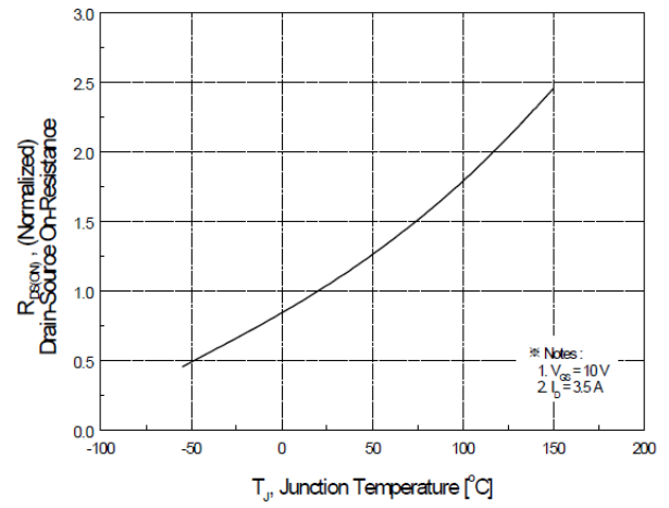
Figure 8. On-Resistance Variation
