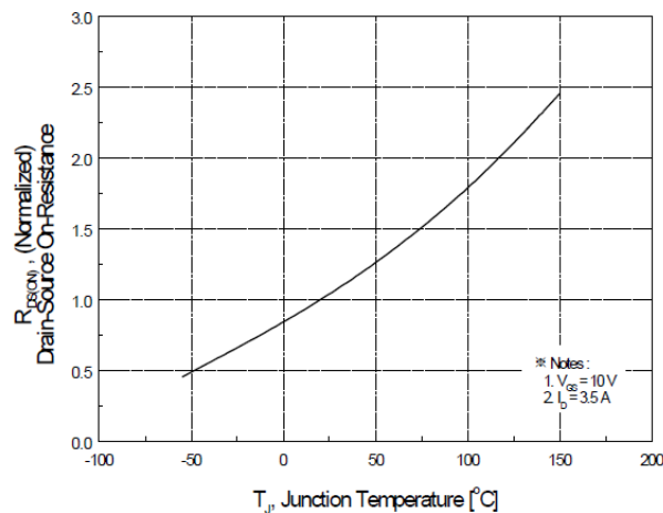
Figure 8. On-Resistance Variation
