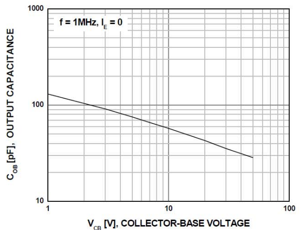
Figure 6. Output Capacitance
