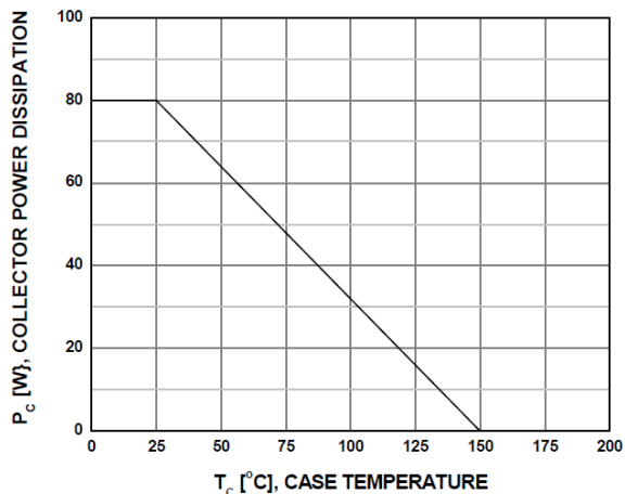
Figure 7. Power Derating
